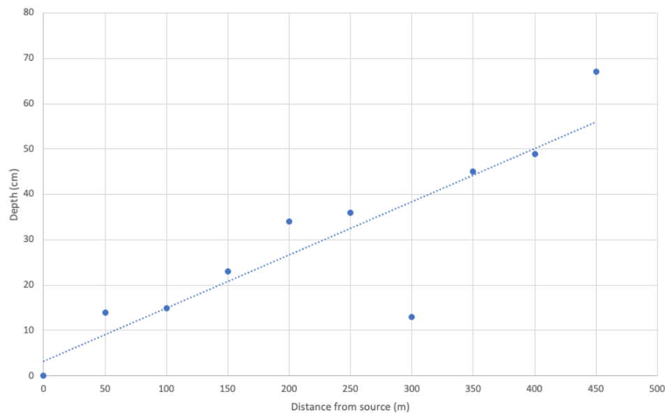
A scatter graph to show the relationship between river depth and distance from source
