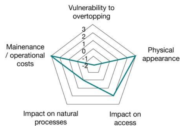
Radar Graph - example
